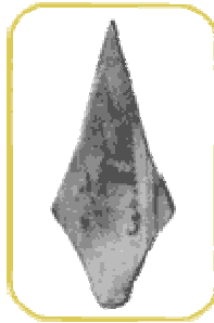
Spear top, concave cast and weld on type 100mm high x 60mm wide Suitable for 12, 14, 16mm round or square vertical bars
