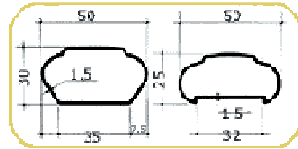
Tube hand rail 50x25x1.5mm x 6m lengths To suit mild steel and tubular steel balustrades
